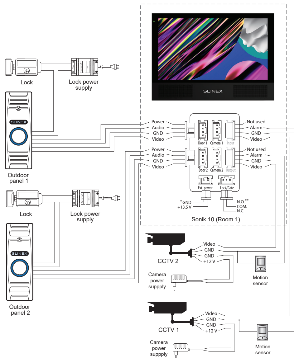
Diagram 1. Sonik 10 outdoor panels, cameras and locks connection.
